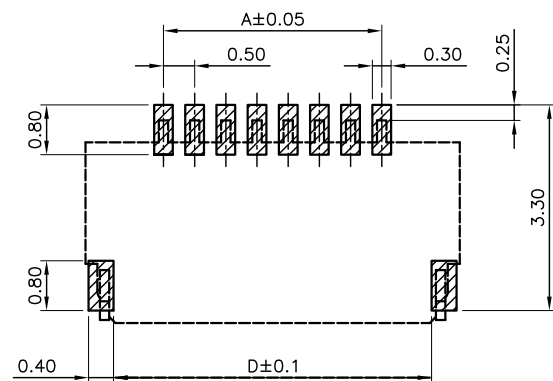
PCB PATTREN LAYOUT
