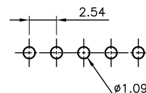
PCB PATTREN LAYOUT
