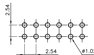
PCB PATTERN LAYOUT
