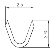
B-B SECTION
