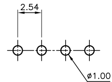
PCB PATTREN LAYOUT
