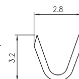
B-B SECTION
