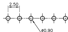
PCB PATTREN LAYOUT
