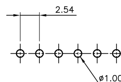
PCB PATTREN LAYOUT
