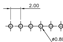
PCB PATTERN LAYOUT
