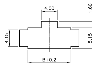
Panel hole dimensions
