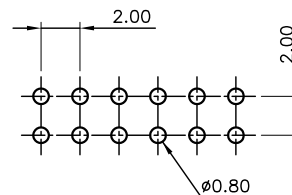
PCB PATTERN LAYOUT
