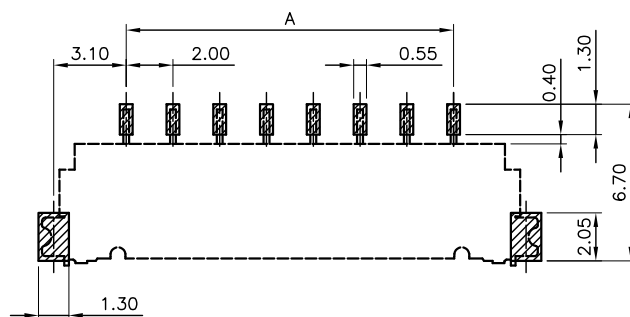
PCB PATTREN LAYOUT
