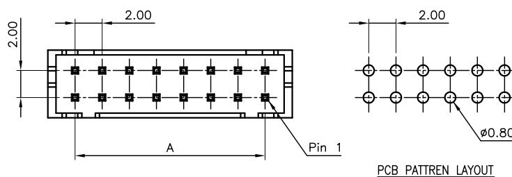
PCB PATTREN LAYOUT
