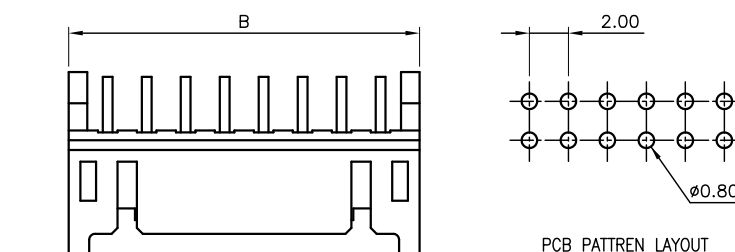
PCB PATTREN LAYOUT
