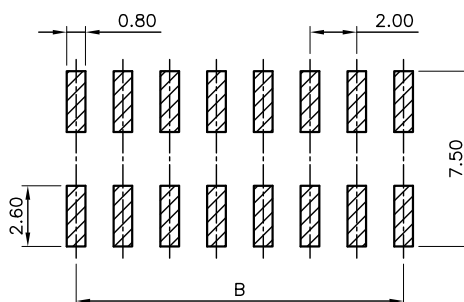
PCB PATTREN LAYOUT
