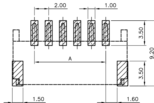
PCB PATTREN LAYOUT
