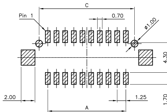
PCB PATTREN LAYOUT
