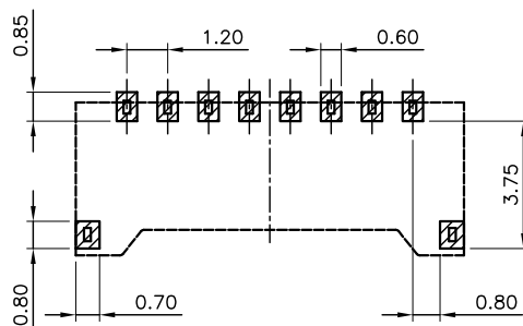
PCB PATTREN LAYOUT
