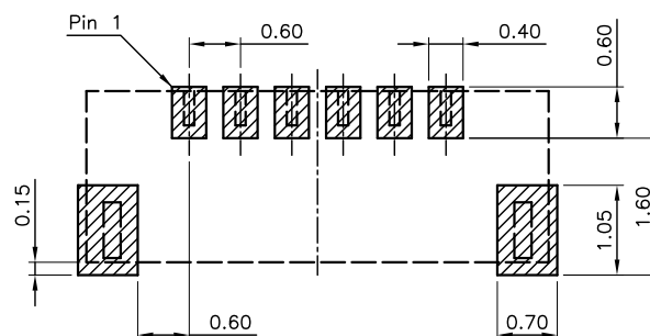
PCB PATTREN LAYOUT
